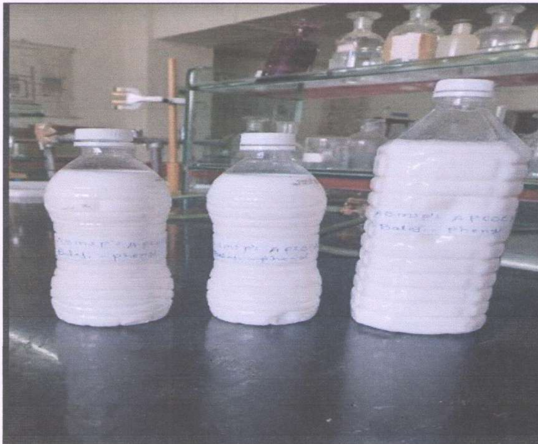
Figure 4. Balaji Phenyl
